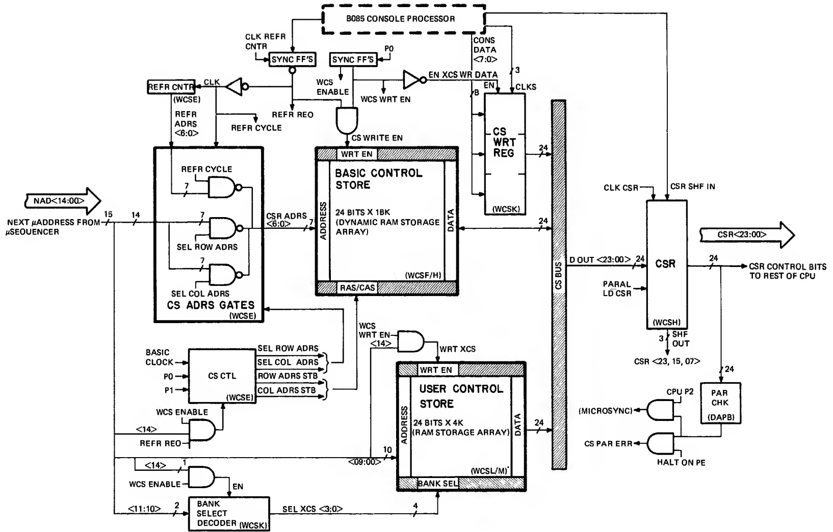
Figure 4-2 Control Store Block Diagram
